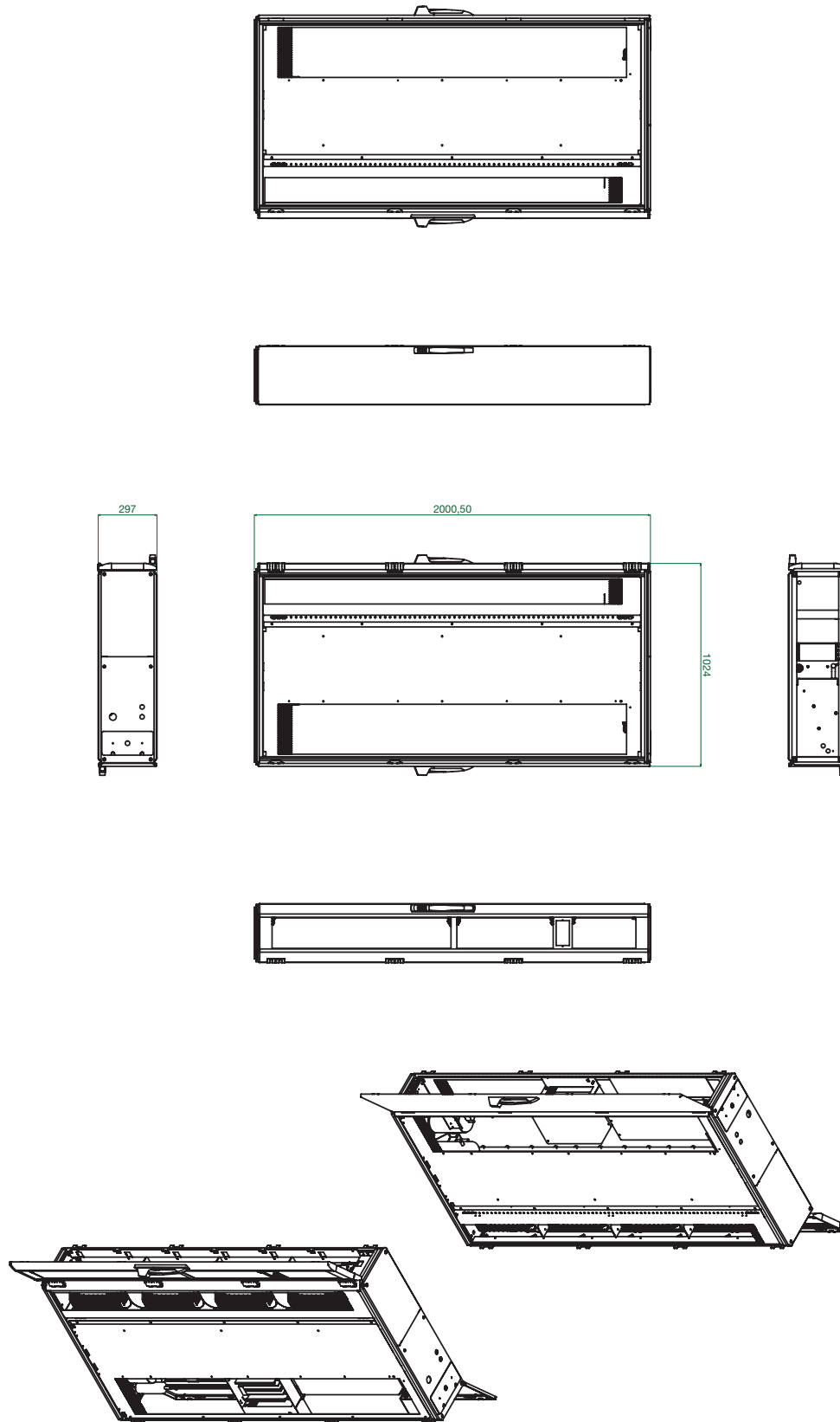
Fig. 45: Overview drawing of the LCP DX (depth 1000 mm)
