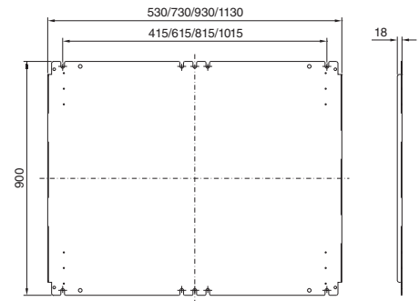
Mounting plate
