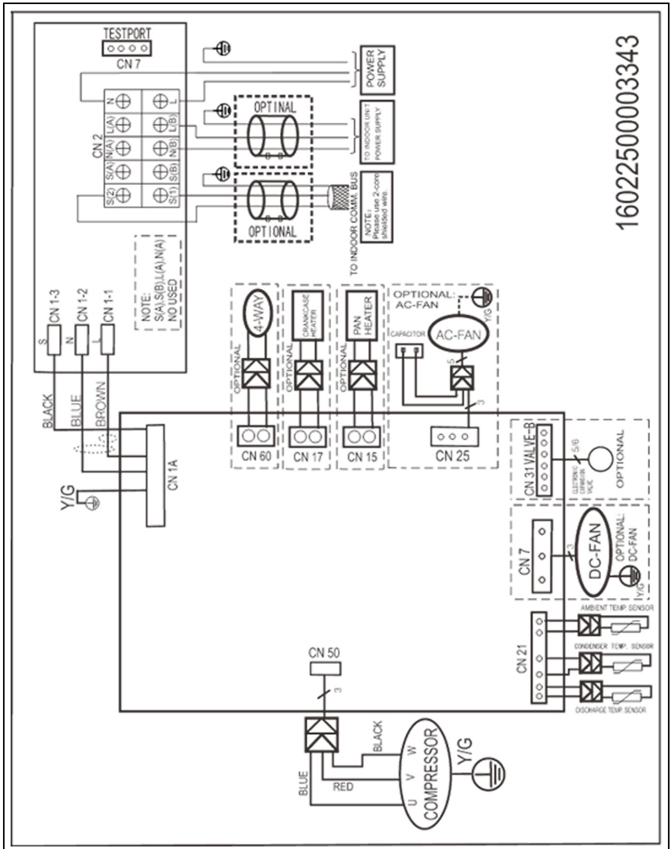
Fig. 25: Circuit diagram, external unit SK 3311.490 and SK 3311.491
