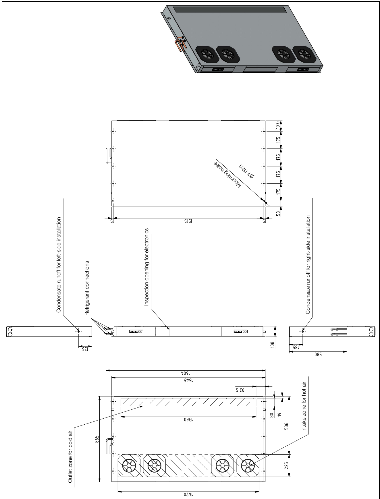
Fig. 21: Dimensions of internal unit LCU DX 3 kW and 6.5 kW
