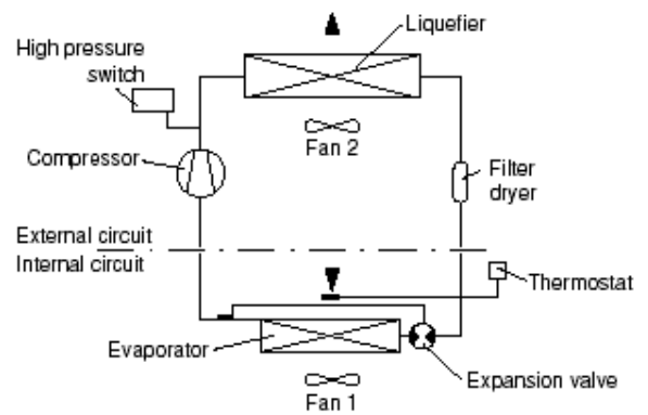
Fig. 8.1 Cooling Circuit
