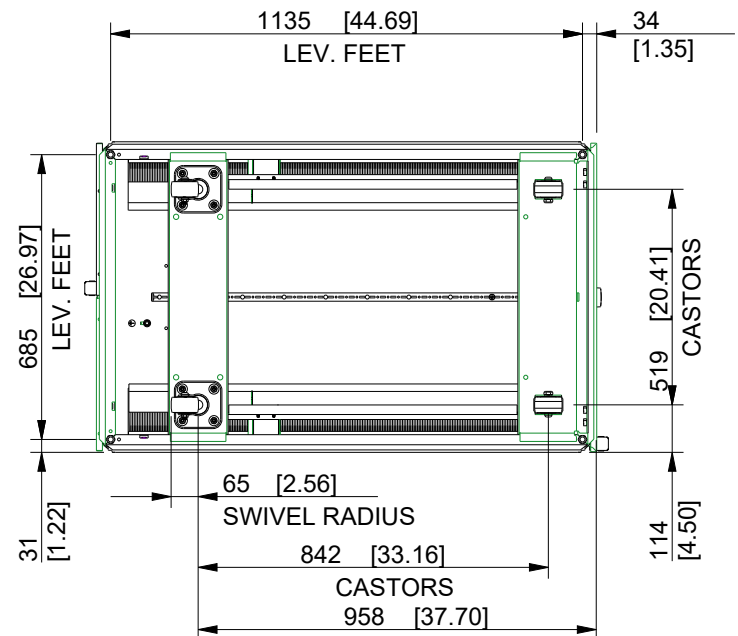
VIEW FROM BOTTOM SHOWING CASTORS AND OPENINGS
