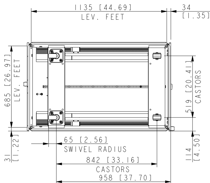
VIEW FROM BOTTOM SHOWING CASTORS AND OPENINGS
