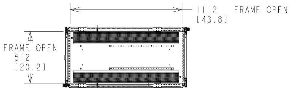
SECTION C-C
