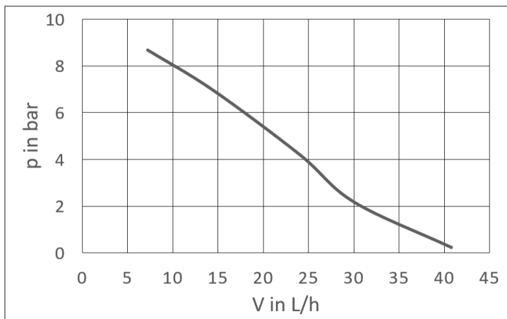
Kennlinie / characteristic curve
