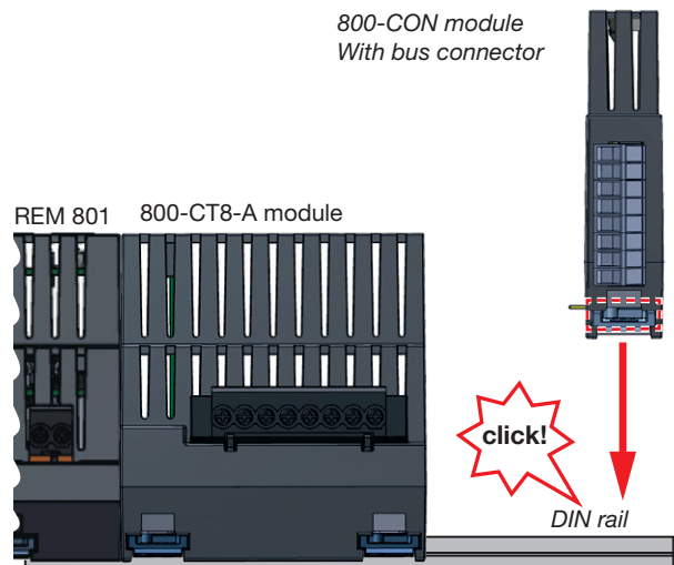
Fig.: Side view, REM 801, 800-CT8-A and 800-CON module
