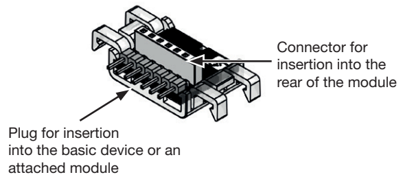
Bus connector for the output transfer module (output bus connector)
