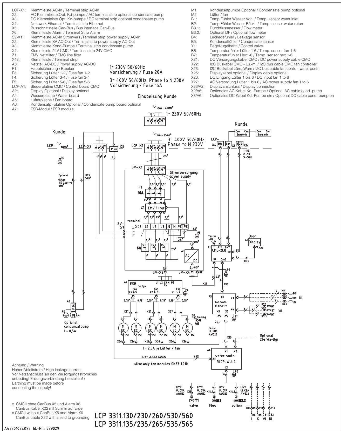
Fig. 111: Circuit diagram LCP Rack/Inline
