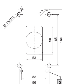
Mounting cut-out
