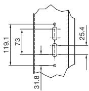
View X
