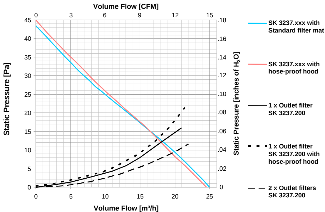
Performance chart SK 3237.xxx [60 Hz]
