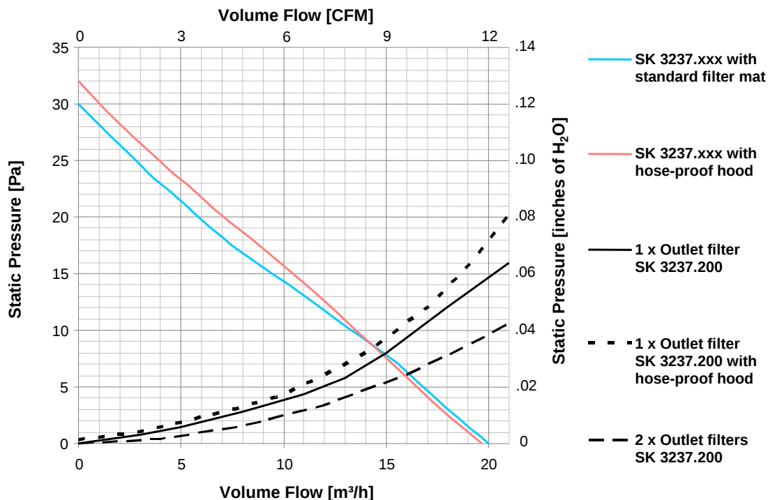
Performance chart SK 3237.xxx [50 Hz]
