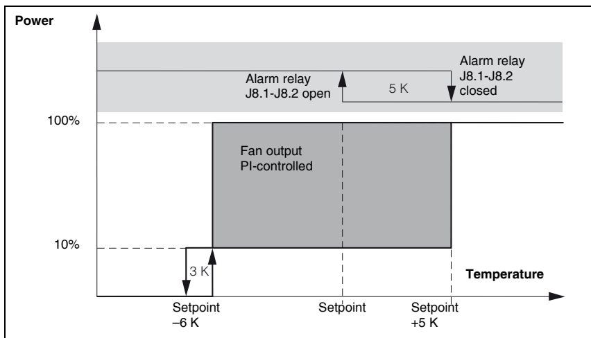
Abb. 1: Temperature control
