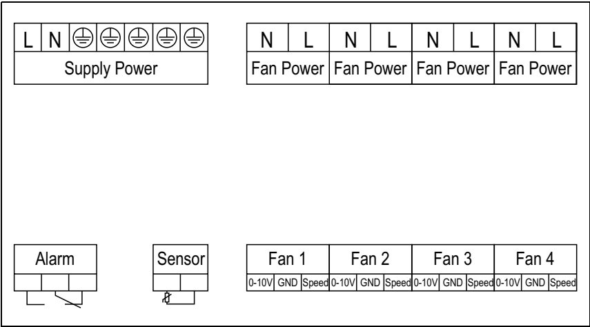
Abb. 2: Electrical connection
