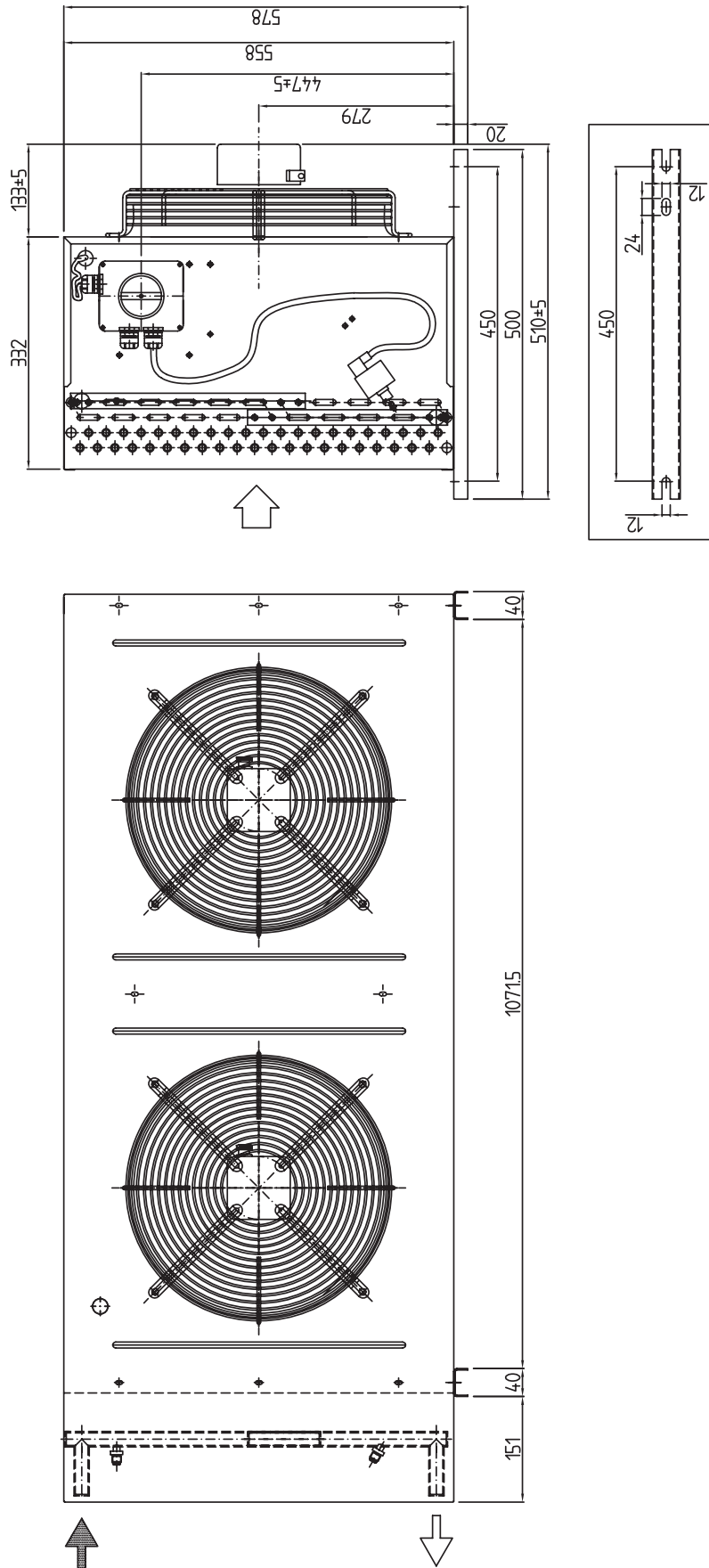
Fig. 50: External condenser (facade mounting)
