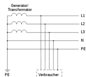
TN-S System
