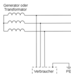
IT System
